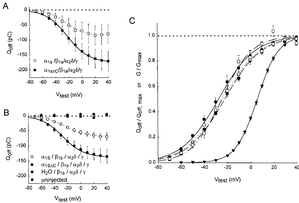
Figure 2. The magnitude and voltage dependence of charge movement in oocytes expressing \alpha_{1S\Delta C} and \alpha_{1S} . (A) Q_{off} versus voltage from five oocytes expressing \alpha_{1S} , \beta_{1a} , \alpha_2\delta , and \gamma ( \square ) and 12 oocytes expressing \alpha_{1S\Delta C} , \beta_{1a} , \alpha_2\delta , and \gamma ( \blacksquare ). The solid and dashed lines through the data points show the mean Boltzmann fits to the data from individual cells (fitted as described in Fig. 1). \alpha_{1S}/\beta_{1a}/\alpha_2\delta/\gamma : Q_{off, max} = -82.9 \pm 32.8 pC, V_{1/2Q} = -24.7 \pm 2.2 mV, k_Q = 13.1 \pm 1.0 mV, n = 5 ; \alpha_{1S\Delta C}/\beta_{1a}/\alpha_2\delta/\gamma : Q_{off, max} = -175 \pm 34.0 pC, V_{1/2Q} = -22.2 \pm 0.8 mV, k_Q = 16.1 \pm 0.3 mV, n = 12 . The differences in Q_{off, max} between these two data sets are not statistically significant ( P = 0.13 ; see text). (B) Q_{off} versus voltage from nine oocytes expressing \alpha_{1S} , \beta_{1b} , \alpha_2\delta , and \gamma ( \circ ), eight oocytes expressing \alpha_{1S\Delta C} ,
